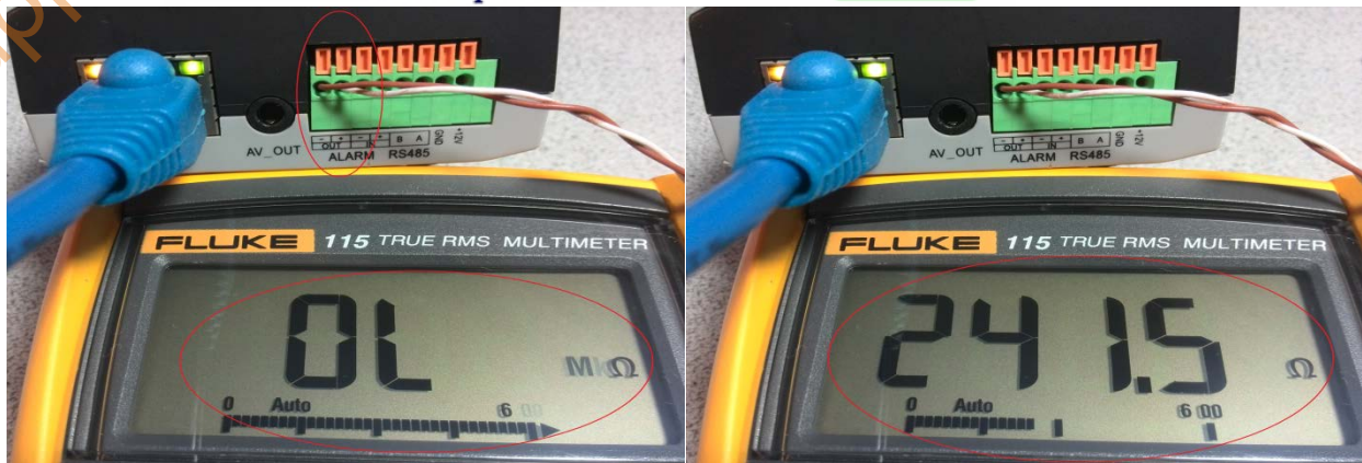
Figure 24-7: Peering GXV3500 Decoder Alarm_Out Circuit
