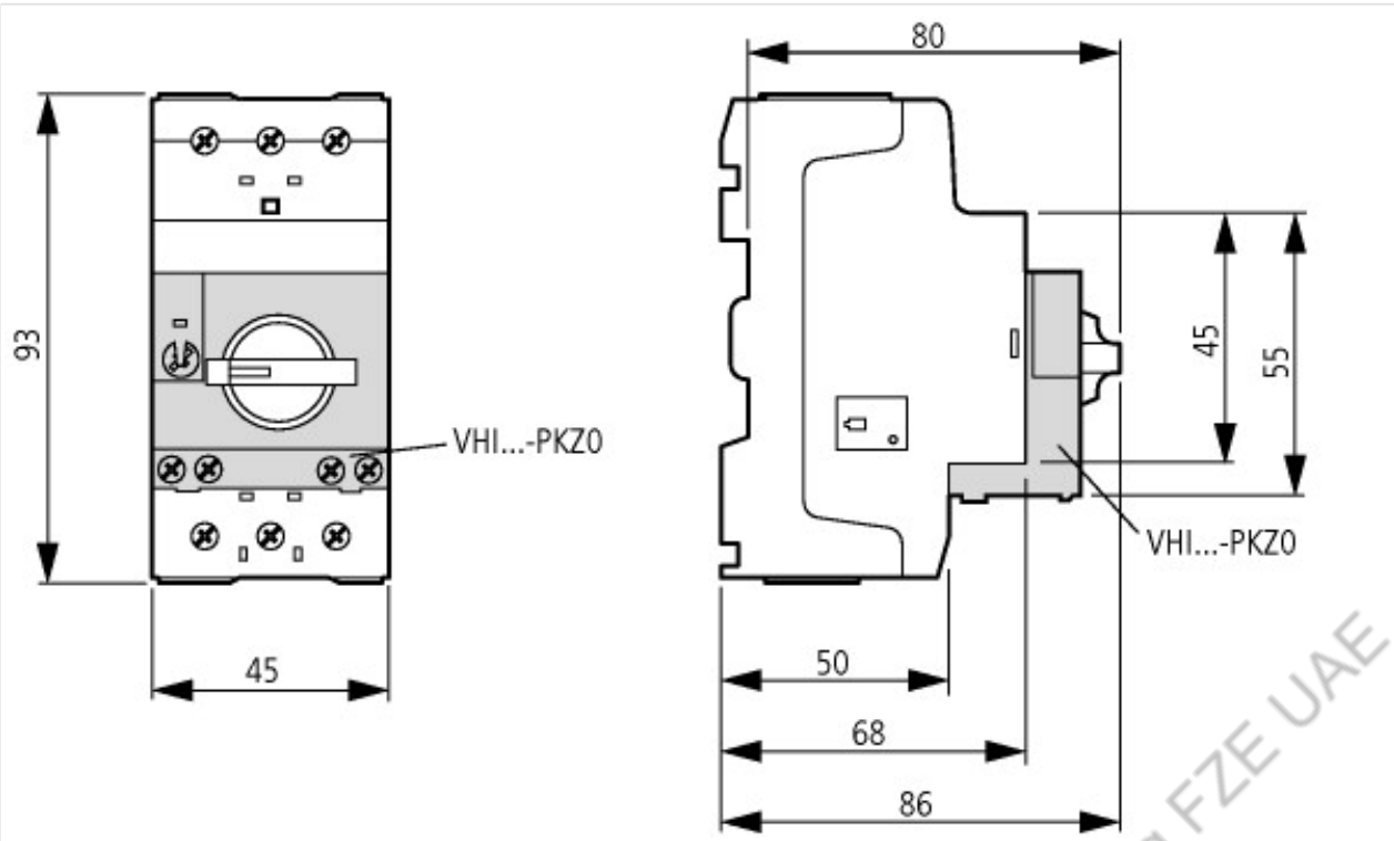
Motor-protective circuit-breakers with early-make auxiliary contacts PKZM0-...+VHI-...-PKZ0
