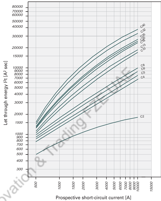
Let-through Energy mRBM, Characteristic C, 1+N-pole
